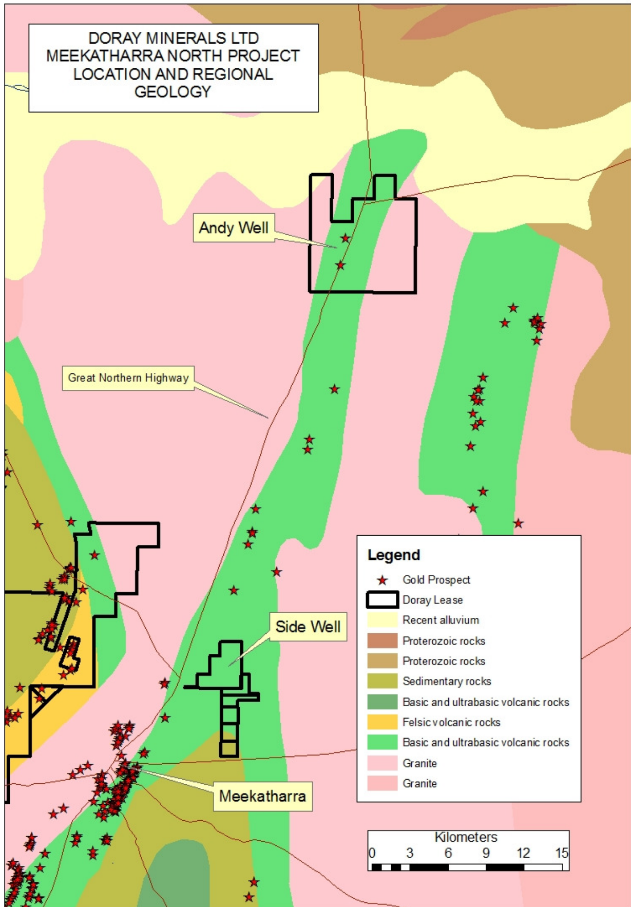
Figure 1. Location of Meeka North and Andy Well, showing gold occurrences and regional geology.
