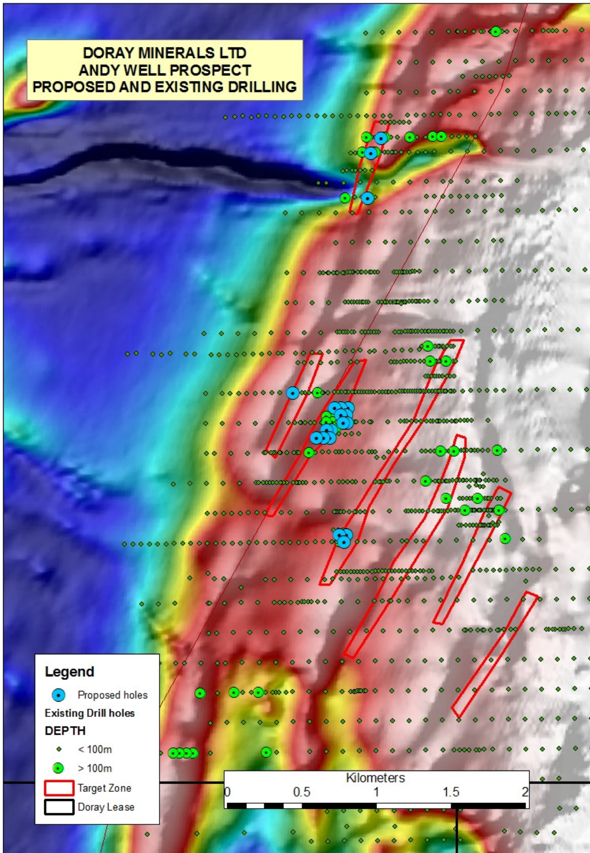
Figure 2. Magnetic image of the Andy Well prospect area, showing previous and proposed drilling in relation to NE-trending mineralised structures.
